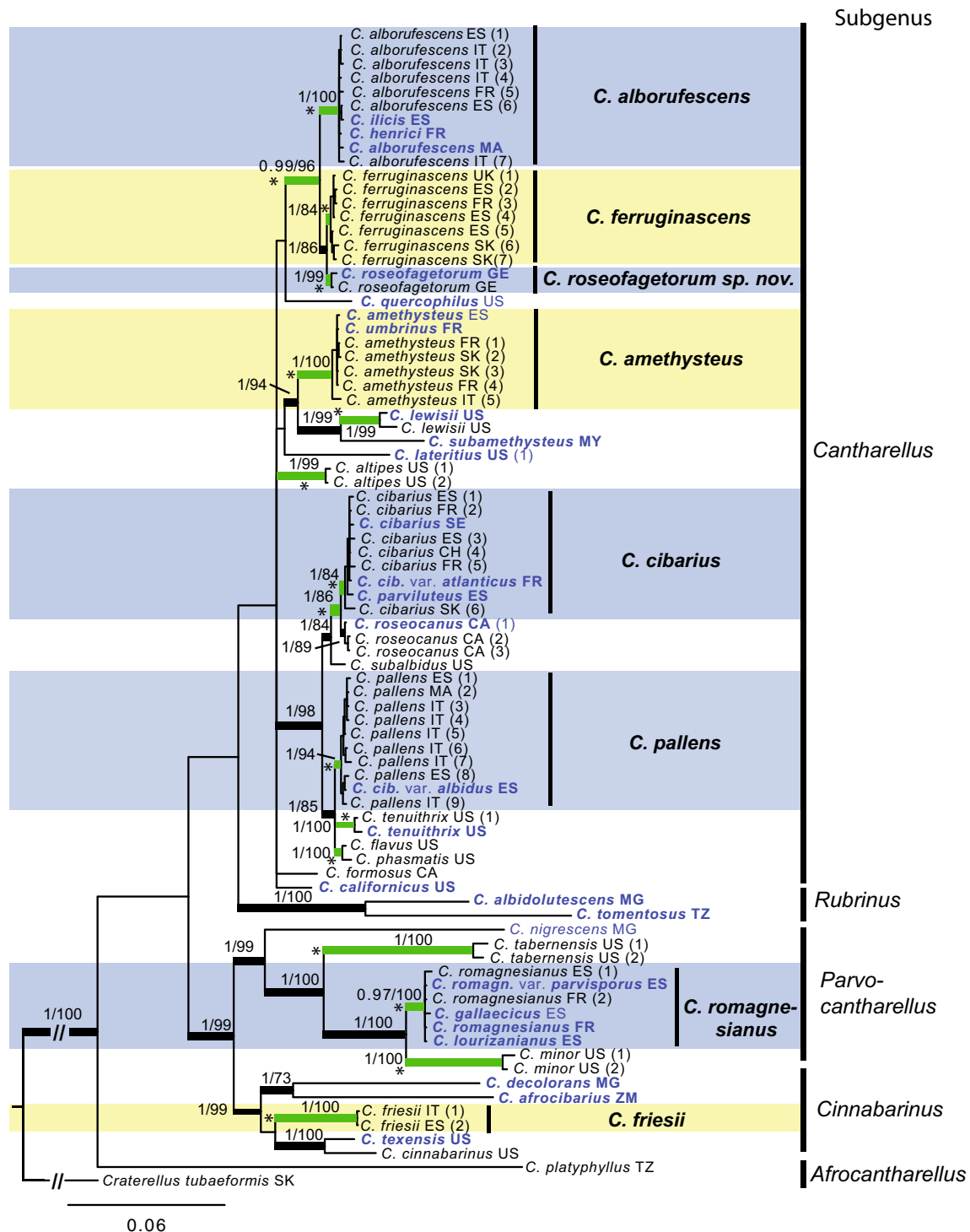
Fig. 1 Bayesian inference 50% majority rule consensus phylogram of Cantharellus from ITS2-LSU-RPB2-TEF-1 sequence data. Bayesian posterior probabilities (PP) \geq 0.95 /Maximum Likelihood bootstrap values (ML-BP) \geq 70\% and are shown by nodes, respectively. Thickened branches received support by both ML-BP \geq 70\% and PP
