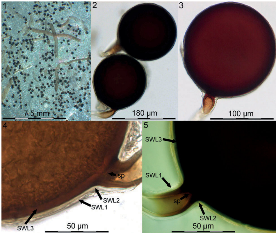
Figs 1–5. Septoglomerus nigrum 1. The dark spores of S. nigrum are formed in trap cultures frequently after > 1 year of cultivation. 2–3. Mature spores are regularly dark brown black to black. 4. Segment of a young, developing spore becoming coffee-brown, while formation of a septum at spore base has started. Spore wall with three layers (SWL1–3). 5. Mature, black spore of S. nigrum . Rarely all three spore wall layers are present on mature spores, as SWL1 is evanescent and short-lived, while SWL2 is semi-persistent, but might also lack completely in older spores.
