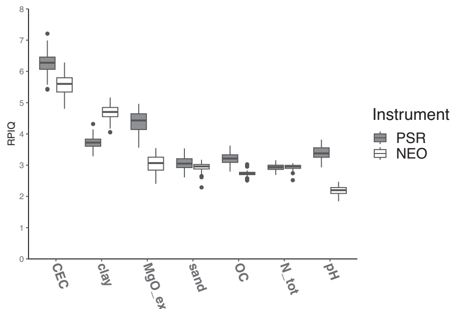
FIGURE 5 Boxplots of the RPIQ (IQR/RMSEP) values of the PSR (full) and the NEO (empty) for the best scanning position (see Table 3).
