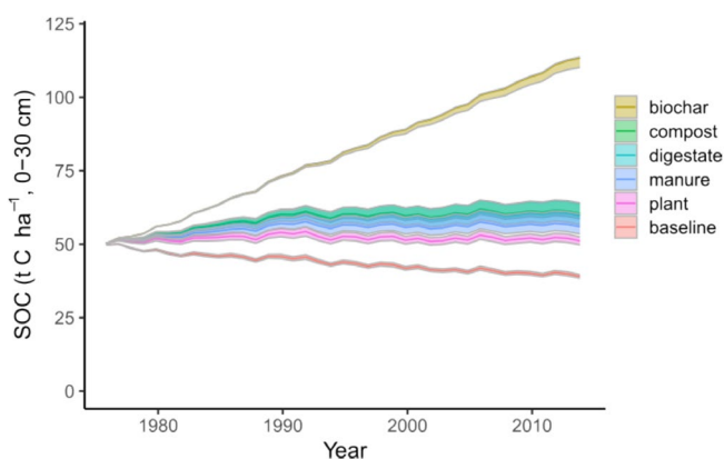
FIGURE 2 | Results of the first analysis presenting the change in soil organic carbon (SOC) stock due to annual additions of 2 \text{ t C ha}^{-1} in the form of different EOMs in addition to only crop residues (baseline) for a Swiss cropland site. Shading represents the area between the upper and lower confidence intervals (reflecting the parameter range).
