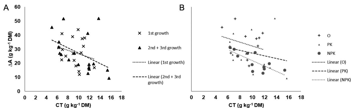
Figure 1. Relationship between condensed tannins (CT) content ( \text{g kg}^{-1} dry matter (DM)) and the increase in protein fraction A from wilted to ensiled forage during the first ( y = -1.26x + 39.4 , P > 0.05 , R^2 = 0.0582 ) or following regrowth ( y = -1.87x + 45.9 , P = 0.05 , R^2 = 0.2193 ) (A) and in relation to type of fertilisation: O: y = -1.38x + 45.9 , P > 0.05 , R^2 = 0.0876 ; PK: y = -0.98x + 36.9 , P > 0.05 , R^2 = 0.0529 ; NPK: y = -1.93x + 41.3 , P < 0.05 , R^2 = 0.5877 (B).
