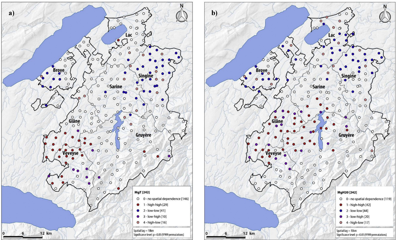
Fig. 3. Cluster map of the Local Indices of Spatial Association (LISA) for (a) Mg_T and (b) Mg_{H2O} with a spatial lag of 10 km. Results are significant at p = .05 (9999 permutations). Five distinct classes (colored circles) are represented: (i) red - high Mg values correlated with high weighted Mg values; (ii) blue - low Mg values correlated with low weighted Mg values; (iii) violet - a low-high relationship between Mg and weighted Mg, (iv) pink - a high-low relationship between Mg and weighted Mg, (v) white - no significant spatial dependence. The background shows the digital elevation model. The lower the altitude, the darker the color. (For interpretation of the references to color in this figure legend, the reader must refer to the web version of this article). Mg forms are determined at 0–20 cm for croplands and 0–10 cm for grasslands and mountain pastures.
