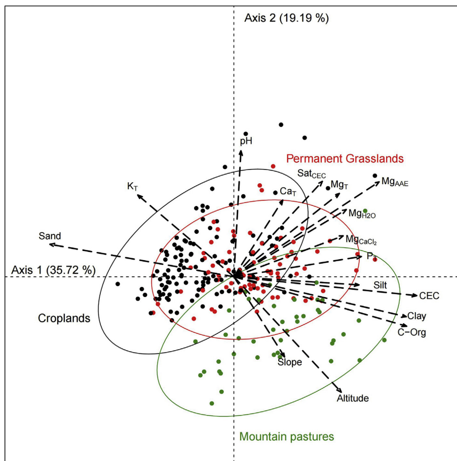
Fig. 2. Principal component analysis of Mg forms, environmental variables and soil characteristics determined at 0–20 cm for croplands and 0–10 cm for grasslands and mountain pastures.
