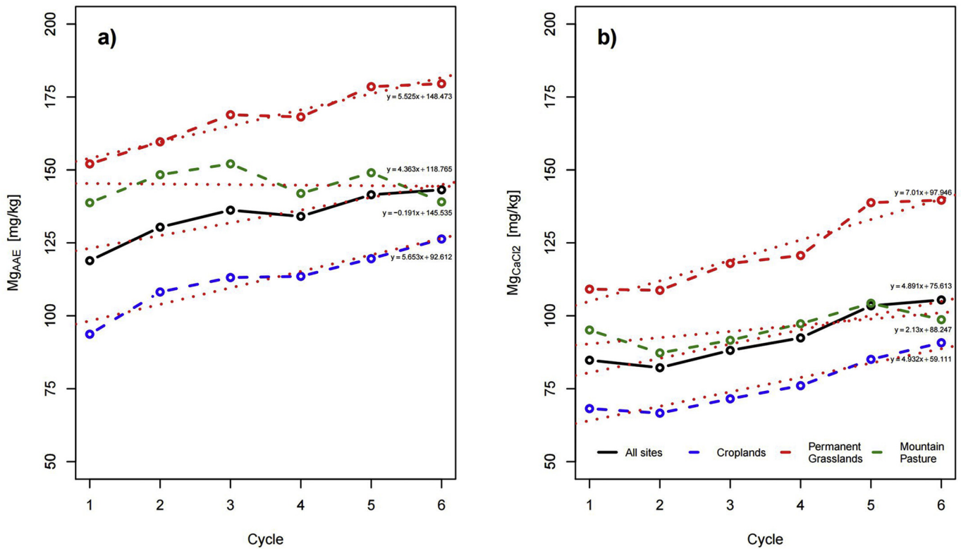
Fig. 5. Temporal changes of (a) ammonium acetate extracted magnesium ( Mg_{AAE} ) and (b) calcium chlorite extracted magnesium ( Mg_{CaCl_2} ) over a 30-year period according to different land use types. Mg forms are determined at 0–20 cm for croplands and 0–10 cm for grasslands, and mountain pastures.
