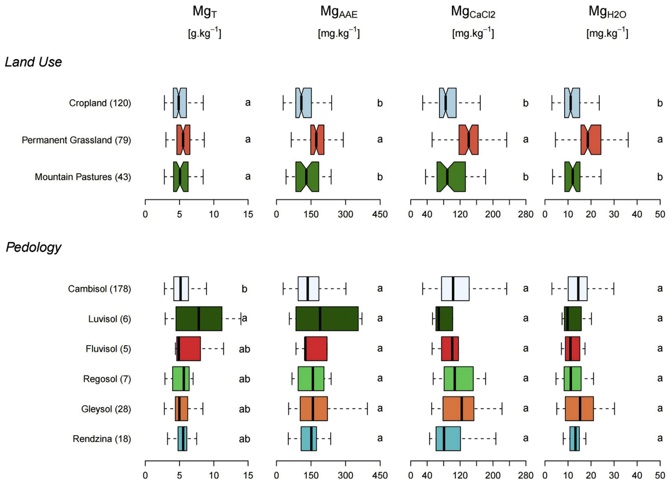
Fig. 1. Boxplots of the different Mg forms in the upper soil layer (0–20 cm for croplands and 0–10 cm for grasslands and mountain pastures) in the FRIBO network according to land use and soil type.
