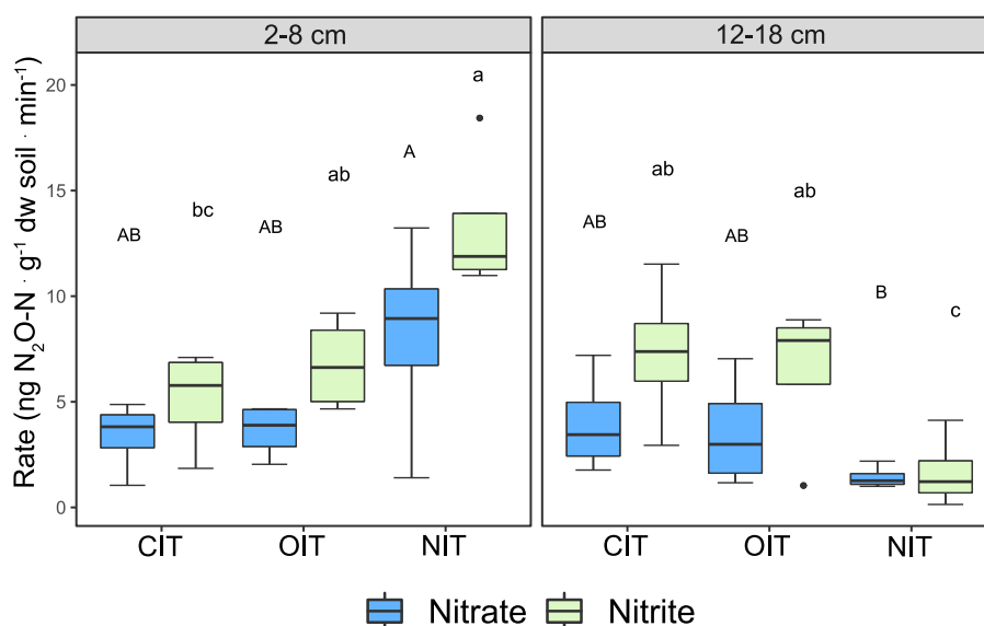
Fig. 1. Potential N 2 O production with addition of NO 3 - or NO 2 - in the upper and lower layer of the topsoil subject to conventional inversion (CIT), occasional inversion (OIT) and non-inversion tillage (NIT). Letters above the boxes indicate statistically significant differences among tillage and depth for each substrate (P < 0.05, n = 4). Upper-case letters represent the comparison among measurements with NO 3 - and lower-case letters show the comparisons of measurements with NO 2 - as substrate.
