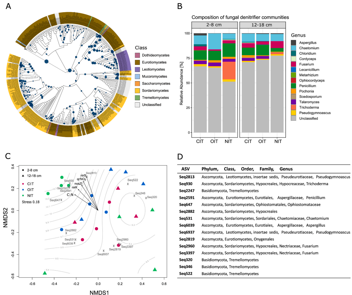
Fig. 3. Fungal denitrifier community structure and composition in the upper and lower layer of the topsoil subject to conventional inversion (CIT), occasional inversion (OIT) and non-inversion tillage (NIT). A) Phylogenetic placements of fungal nirK amplicon sequence variants within a fungal nirK phylogeny of 375 taxa and 42 bacterial, 5 archaeal and 26 multicopper oxidase leaves as the outgroup. The outer ring is coloured according to the taxonomic class. Taxa with unknown taxonomic rank are underlined in white. The majority of fungal nirK placements fall in the class Eurotiomycetes (brown), Sordariomycetes (yellow), Leotiomyces (purple) and Tremellomycetes (green). B) Relative abundances of fungal genera assigned by the placement of nirK sequences by tillage treatment and soil depth. 'Unclassified' refers to sequences that could not be assigned at the genus level. C) Non-metric multidimensional scaling (NMDS) of the fungal denitrifier community based on fungal nirK ASVs with smooth response curves of a distinct gradient of C:N ratio that varied across the treatment depending on depth using the function ORDISURF. Colours indicate tillage regime, and shape depicts soil depth. The arrows show significant correlations ( P < 0.01 ) of denitrification genes and NO 2 - -induced denitrification rates with the fungal community structure, with the direction indicating a positive correlation, and grey crosses represent significantly correlated ASVs (999 permutations). D) Taxonomic lineages of nirK ASVs contributing to the sample distribution in the NMDS.
