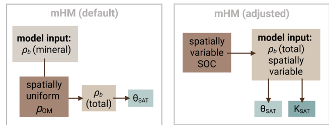
Figure 2. Adjustment of bulk density ( \rho_b ) for organic matter ( \rho_{\text{OM}} ) in the default mHM routine, compared to the model version adapted for this study using spatially distributed SOC data.
