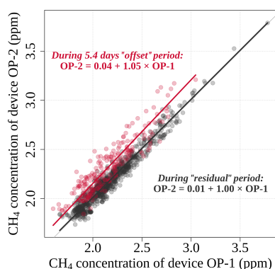
Figure 5. Scatter plot of 30 min data from OP-1 and OP-2 recorded during campaign A18. Deming regression lines and corresponding regression equations are shown for the offset period and the remaining (“residual”) period.
