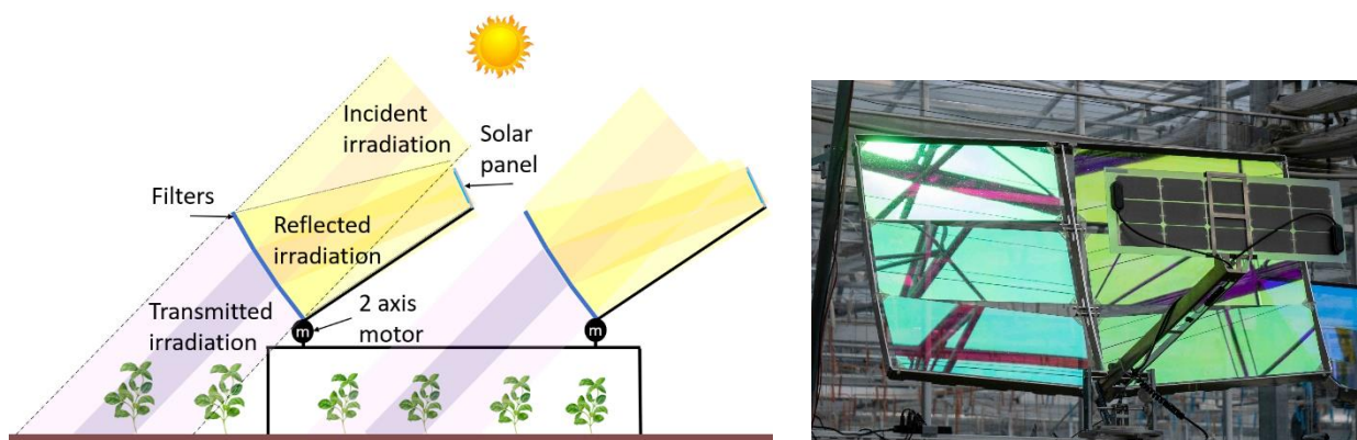
Figure 1: Schematic of the Voltiris system and photograph of the 6-fold concentration (X6) system in the experimental greenhouse.
