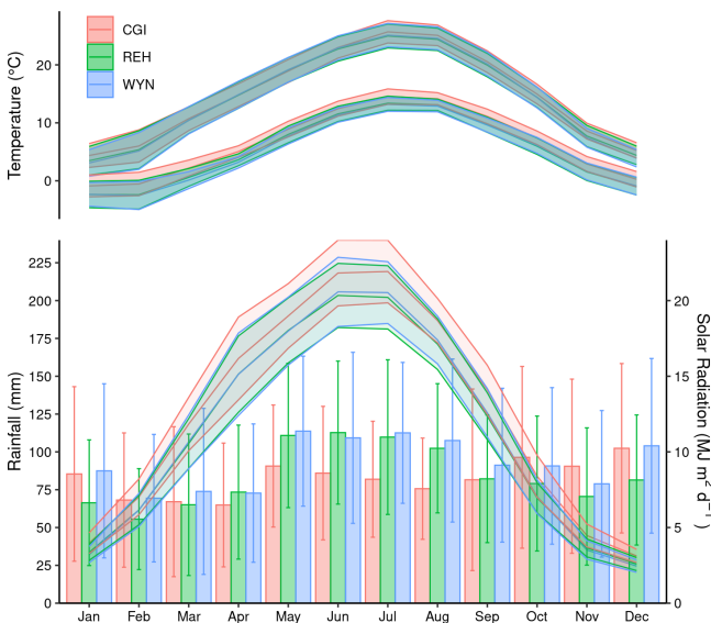
Figure 1. Seasonal variability of climatic variables considering monthly mean \pm standard deviation (shades and bars) values observed at the meteorological stations between 1981 and 2022. Rainfall corresponds to monthly sums, while other variables represent daily values averaged by month. Minimum (bottom lines) and maximum (upper lines) temperatures are presented.
