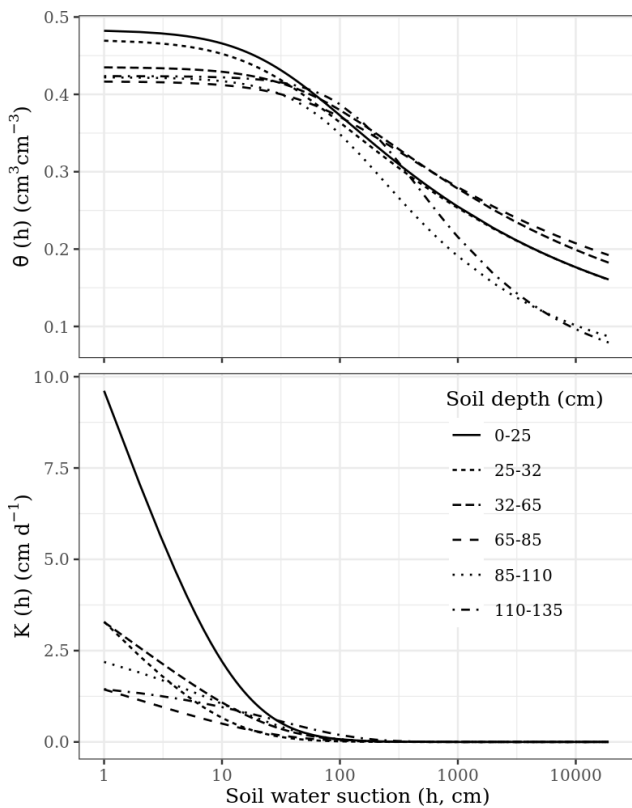
Figure 3. Soil water retention ( \theta ) and soil hydraulic conductivity ( K ) as functions of the soil water suction ( h ) at the evaluated soil profile estimated by the euptfv2 (option PTF02).
