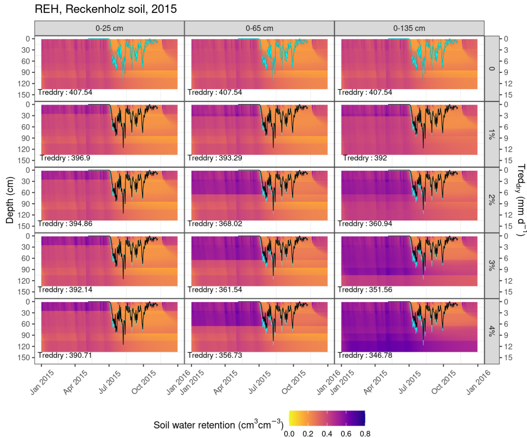
Figure 6. Detailed profile of soil water content (left axis) and Tred_{dry} (right axis, black lines) according to the different added SOC levels at the Reckenholz site (REH) in the year of 2015. The blue line represents Tred_{dry} for the original soil profile (0 % SOC). When cumulated for the year, their difference yields the annual ATG in crop transpiration deficit that is due to the addition of carbon to the soil.
