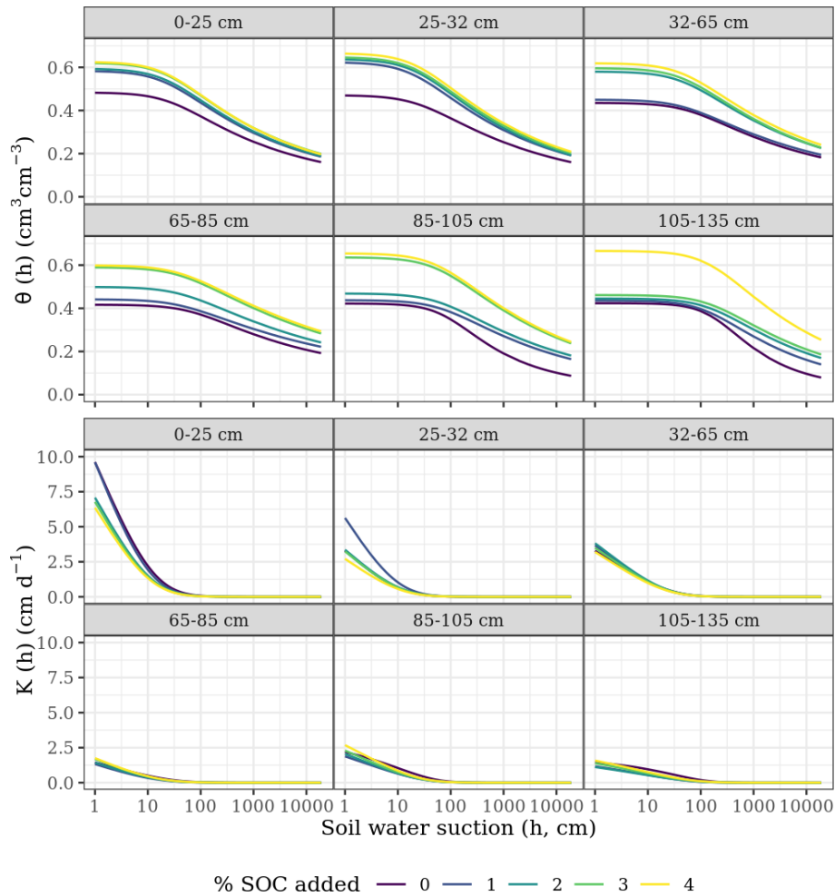
Figure 4. Effects of SOC increase on the soil water retention ( \theta ) and soil hydraulic conductivity ( K ) as functions of the soil water suction ( h ) as predicted by euptfv2, option PTF02.
