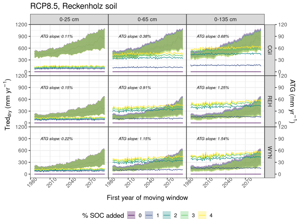
Figure 5. Transpiration reduction due to drought stress ( Tred_{dry} ) (left axis, green band) for actual and future climate conditions considering different levels of SOC increase in the soil at different effective soil depths and average transpiration gain, ATG, (right axis, coloured lines) between 0 % and 4 % addition of SOC. Climate projections considered the RCP8.5 pathway and were averaged for every 10 years. The green shaded area of Tred_{dry} refers to the values between the (dotted) quantiles q_{0.05} and q_{0.95} of the climate projections. ATG is interpretable as average seasonal gain in transpiration due to SOC increase, and ATG slope refers to the slope of the ATG line between 0 % and 4 % SOC addition.
