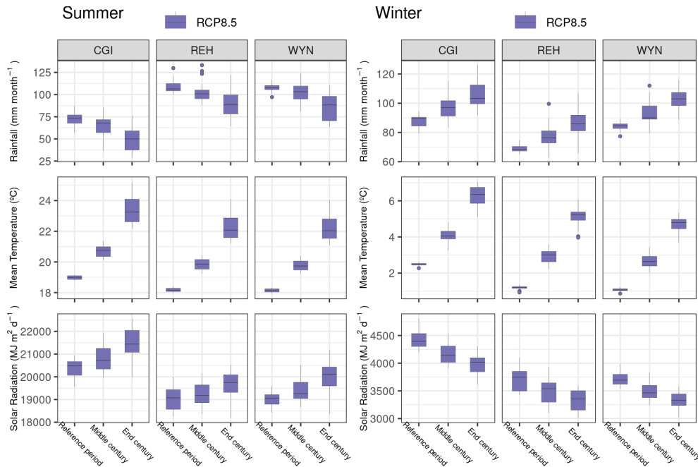
Figure 2. Summary of climatic variables considering monthly mean values at the stations Changins (CGI), Reckenholz (REH), and Wynau (WYN) for the projections of RCP8.5. Summer was considered to be the months of June, July, and August, and winter corresponds to December, January, and February. Reference period: 1981–2020, mid-century: 2031–2060, end of century: 2071–2099. Rainfall corresponds to monthly sums, mean temperature is the mean between the maximum and minimum temperatures per day averaged by month, and solar radiation corresponds to daily values averaged by month.
