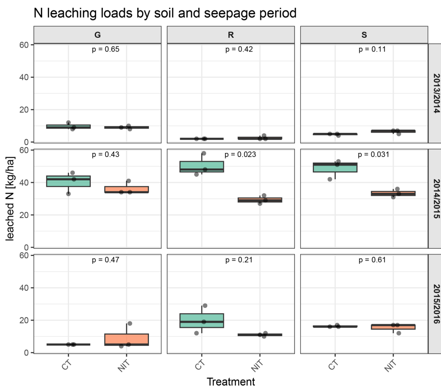
Figure 2. Boxplots of cumulative \text{NO}_3^- -N loads leached from lysimeters by seepage period, soil (G = Cambisol from Grafenried, R = Stagnic Cambisol from Reckenholz, S = Luvisol from Schafisheim) and by treatment (NIT = non-inversion tillage with chisel plough, CT = conventional tillage with mouldboard plough); n = 18 (2 treatments \times 3 soils \times 3 replicates)).
