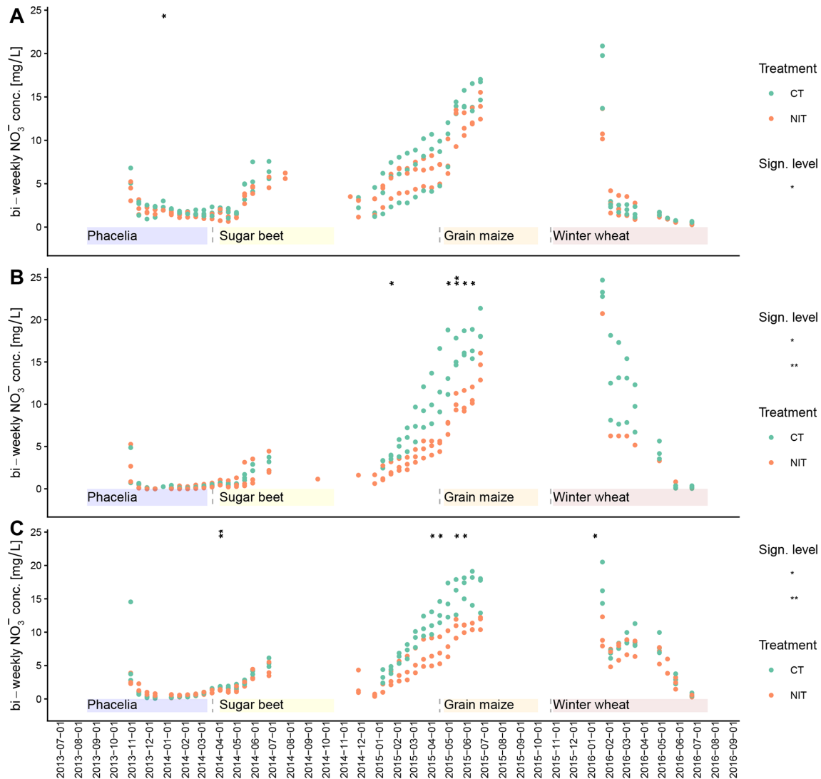
Figure 4. Time series of bi-weekly \text{NO}_3^- concentrations in seepage water from lysimeters of both treatments (CT = conventional tillage, NIT = non-inversion tillage) by soil type (A = Cambisol from Grafenried, B = Stagnic Cambisol from Reckenholz, C = Luvisol from Schafisheim); coloured shading is in reference to cropping periods: purple (phacelia), yellow (sugar beet), orange (grain maize), red (winter wheat); grey dashed vertical lines denote ploughing times; stars indicate statistical significance of treatment differences ( p -value < 0.01 “***”; p -value < 0.05 “**”); n = 18 .
