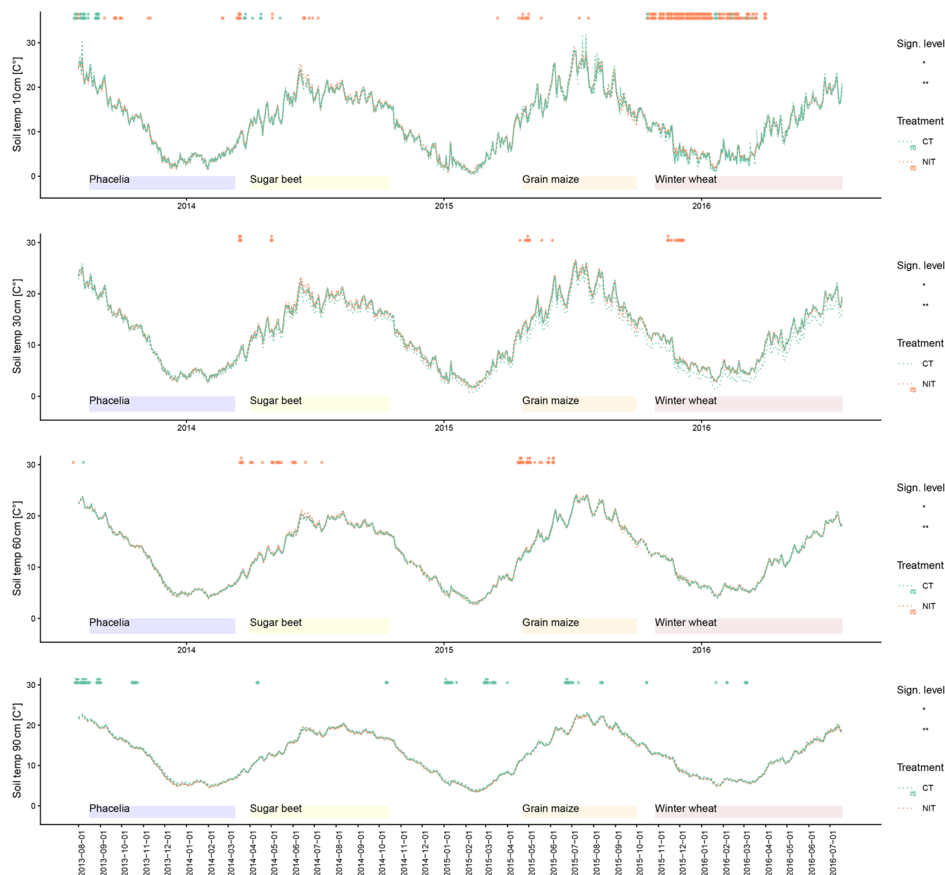
Figure C3. Soil temperatures recorded in four depths in three lysimeters by treatment (NIT = non-inversion tillage, i.e. chisel plough; CT = conventional tillage, i.e. mouldboard plough); stars indicate statistical significance of treatment differences ( p -value < 0.01 “**”, p -value < 0.05 “*”), colours of asterisks indicate direction of treatment difference: higher temperatures in NIT are indicated by red asterisks, higher temperatures in CT are indicated by green asterisks); n = 12 (2 treatments \times 3 soil types \times 2 sensor replicates).
