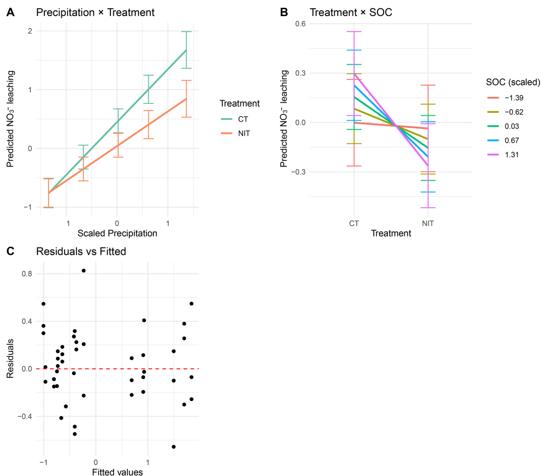
Figure 11. Modelled interactive effects between precipitation and treatment (A), treatment and SOC (B) on \text{NO}_3^- leaching and residual plot of the fitted model (C).
