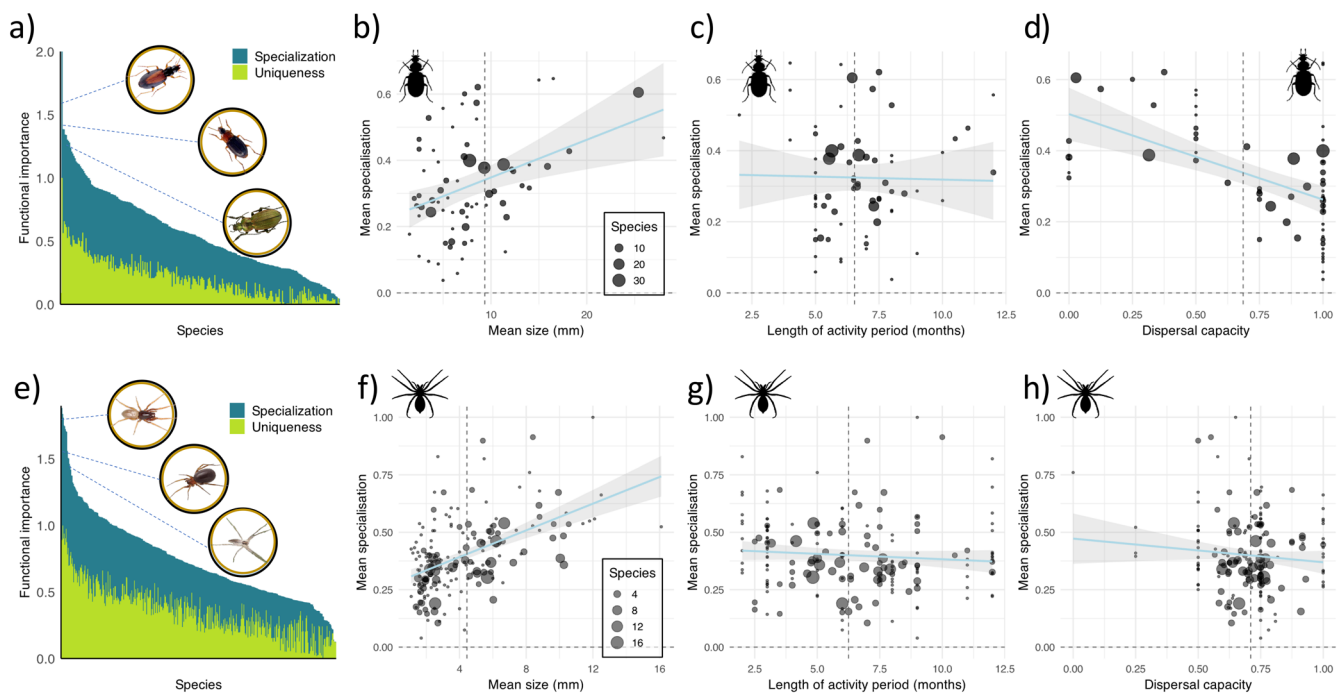
FIGURE 5 | Species and trait contribution to functional richness. Ranking of carabid (a) and spider (e) species by their functional importance, expressed as the sum of normalised (0–1) uniqueness (distance to k nearest neighbours; light green) and specialisation (distance to the centroid; blue). Bars represent the aggregated contribution of each species to overall functional diversity. Example species contributing most to functional richness are illustrated. Carabids: Dolichus halensis (photo by U. Schmidt; https://species.wikimedia.org/ ), Calathus melanocephalus and Carabus monilis (photos from https://www.coleoptera.org.uk , by Lech Borowiec). Spiders: Dysdera erythrina (photo by Arno Grabolle), Zodarion italicum (photo by Ulrich Kursawe) and Pisaura mirabilis (photo by Luis Nunes Alberto; https://commons.wikimedia.org/ ). Association between mean specialisation and genus-level mean traits, including body size (b, f), length of their activity period (c, g) and dispersal capacity (d, h), for carabids and spiders, respectively. Vertical dashed lines show the average value of traits across genera. Fitted lines represent linear models with 95% CIs. See Figure S12 in Supporting Information for the degree of functional specialisation, including all the genera with more than one species in our dataset.
