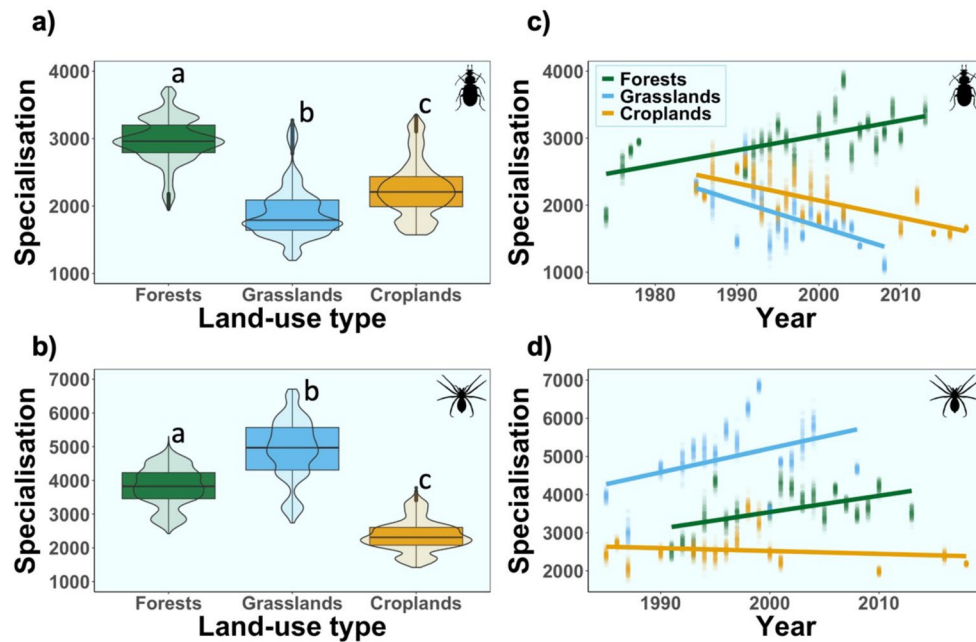
FIGURE 2 | Variation in assemblage functional specialisation across years and land-use types. Variation in (a) carabid, and (b) spider functional specialisation assemblage-weighted means across land-use types. Temporal trends of (c) carabid and (d) spider functional specialisation within each land-use type (c. Letters in panels a) and (b) show post hoc Tukey significant differences between groups. All the trends in panels (c, d) were significant (95% CI of the slope not including 0) and significantly different from each other.
