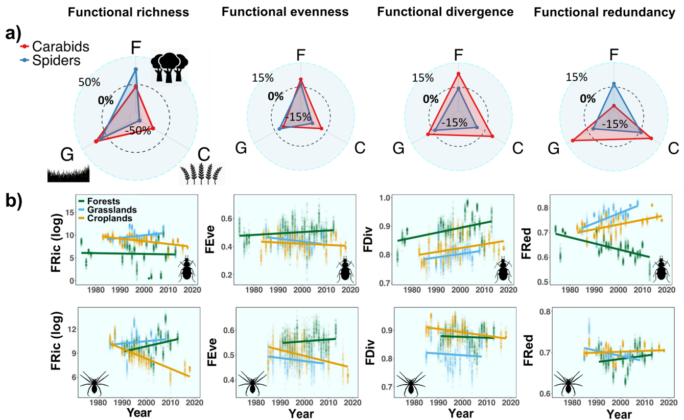
FIGURE 1 | Temporal trends in overall functional diversity of carabid and spider assemblages across three land-use types. (a) Rate of change per decade in three land-use types: F = forests, G = grasslands, C = croplands. (b) Linear fit showing the marginal effect of year (i.e., temporal trend) on carabid (top) and spider (bottom) functional richness (FRic), functional evenness (FEve), functional divergence (FDiv) and functional redundancy (FRed) across three land-use types. These metrics were calculated from functional distances based on the full set of traits (i.e., including response and effect traits).
