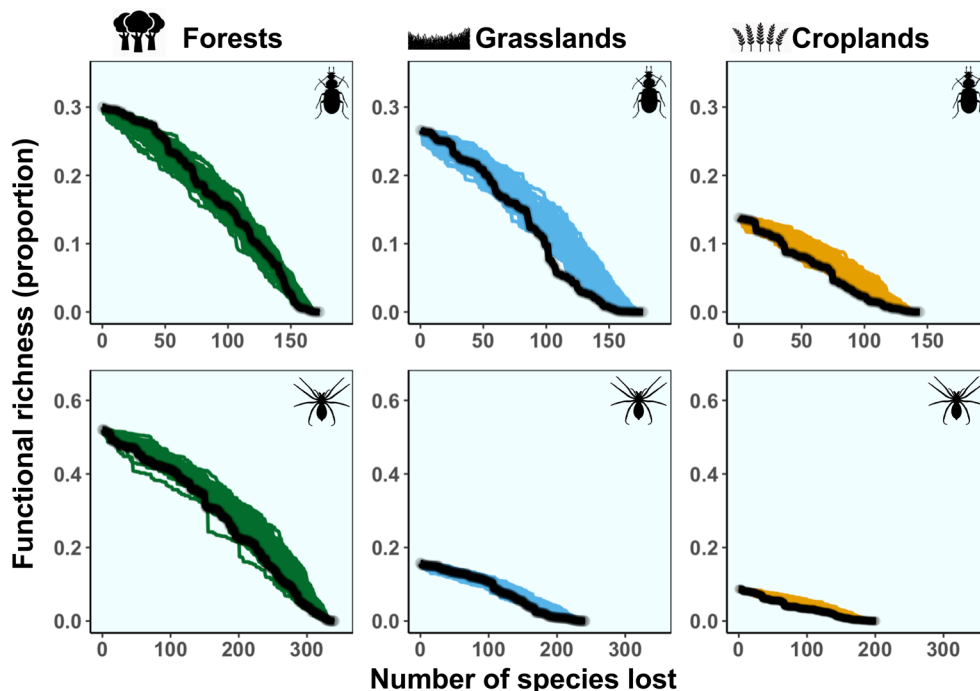
FIGURE 4 | Decrease in functional richness under different scenarios of carabid and spider species loss in forests, grasslands, and croplands. Decline rate of the functional richness space occupied by the species found in forests, grasslands, and croplands, as species are removed randomly (coloured lines, 50 iterations) or in abundance increasing order (i.e., from less abundant to more abundant) (black line). Functional richness is expressed as the proportion of the total trait space defined by all species found in the dataset. Initial values are < 1 because not all species occur within a single land-use type. Notice that the scale of the Y-axes of carabid beetles and spiders is different.
