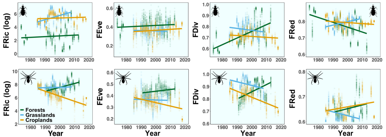
FIGURE 3 | Temporal trends in functional diversity based on three key effect traits. Each panel includes three land-use types: Forests (green), grasslands (blue) and croplands (orange). The effect traits used to define functional distances were body size, phenology duration and feeding guild (carabids)/hunting technique (spiders). FRic = functional richness, FEve = functional evenness, FDiv = functional divergence, FRed = functional redundancy. These metrics were calculated from functional distances based on three effect traits.
