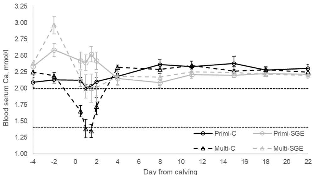
Fig. 2. Blood serum calcium concentration (least square means ± SE) in periparturient primiparous (Primi) and multiparous (Multi) cows given, four days prior to calving, a rumen bolus containing 0 (C) or 500 (SGE) µg 1,25(OH) 2 D 3 , provided as 1,25(OH) 2 D 3 glycosides from S. glaucophyllum . Parity ( P < 0.05 ), Bolus ( P < 0.01 ), Day ( P < 0.001 ) and Parity × Bolus × Day ( P < 0.001 ). The limits for clinical and subclinical hypocalcaemia (<1.4 and <2.0 mmol/l, respectively) are indicated as dotted lines.
