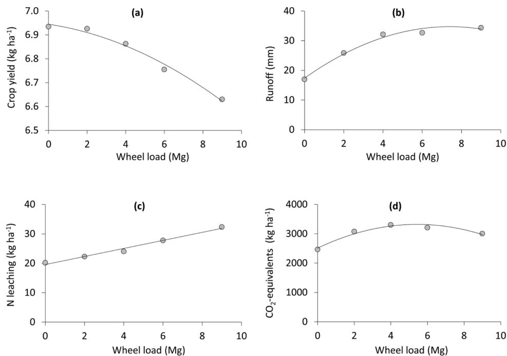
Fig. 2. (a) Impact of soil compaction, expressed in terms of harvester wheel load, on (a) crop yield, (b) surface runoff, (c) nitrogen leaching, and (d) greenhouse gas emissions.
