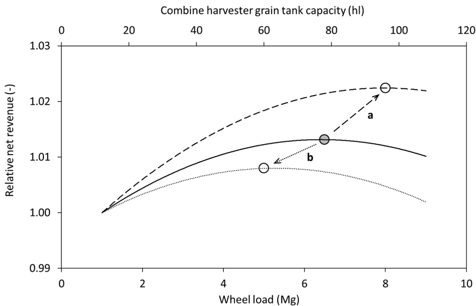
Fig. 4. Relative changes in farmer net revenue as a function of wheel load for three different scenarios; for each scenario, calculations with 1 Mg wheel load serve as reference (relative net revenue = 1.0). Solid curve: baseline scenario, i.e. as in Fig. 3a; dashed curve: 15% lower producer price; and dotted curve: 15% higher producer price. Optimal harvester size for maximum private profit of farmer is indicated for each scenario by circles. Lower producer prices result in larger optimum harvester size (a), while higher producer prices result in smaller optimum harvester size (b).
