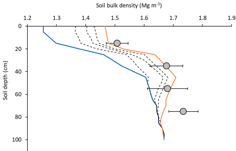
Fig. 1. Simulated soil bulk density (lines) as a function of soil depth for different wheel loads corresponding to different harvester sizes (blue: no compaction, i.e. 0 Mg wheel load; orange: modern harvester with 9 Mg wheel load; black dashed curves: 2, 4 and 6 Mg wheel load), and measured soil bulk density (symbols) in a farmer’s field in Scania county. Error bars represent standard deviation of mean.
