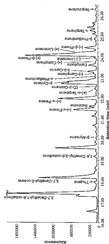
Figure 1 GC-MS total ion chromatogram (TIC) depicting the monoterpene range of milk
