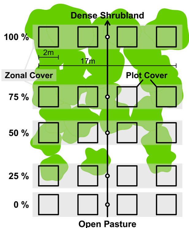
Fig. 2 Schematic representation of the sampling approach along a transect from open pasture to dense shrubland. The arrow represents the centre line along the transect. Small circles along the arrow indicate poles in five zones with estimated zonal cover of 0, 25, 50, 75 and 100%. Quadrates show four sampling plots of 2×2 m at fixed distances along lines perpendicular to the pasture-shrub transect. A value of plot cover was assessed for each sampling plot
