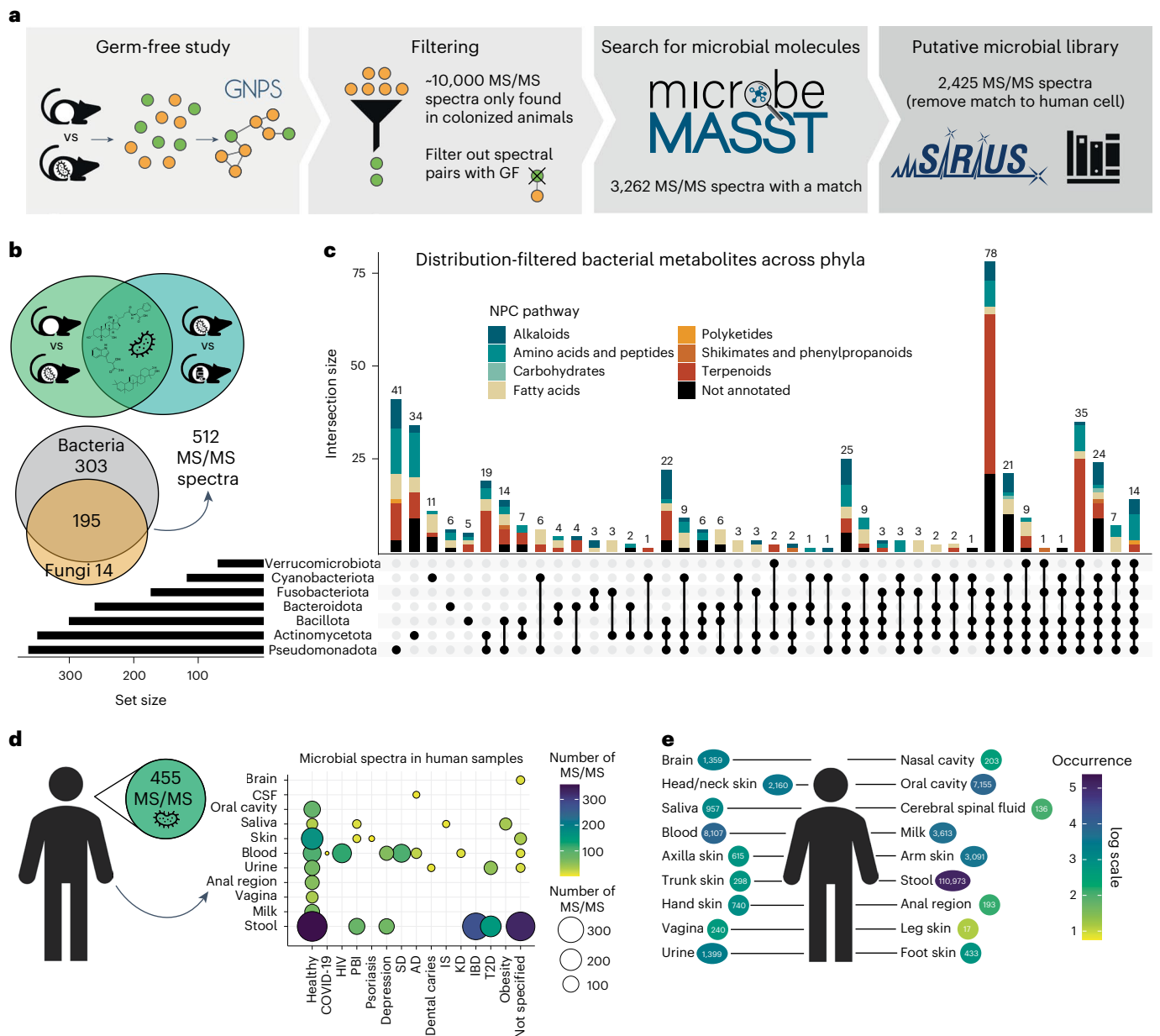
Fig. 2 | microbeMASST can identify microbial MS/MS spectra within mouse and human datasets. a , Workflow to extract microbial MS/MS spectra from biochemical profiles of 29 different tissues and biofluids of SPF mice that are not observed in GF mice 30 . The MS/MS spectra unique to SPF mice (10,047) were searched with microbeMASST. A total of 3,262 MS/MS spectra had a match; those MS/MS also matching human cell lines were removed, leaving a total of 2,425 putative microbial MS/MS spectra (see Methods to download .mgf file). b , The presence of the 2,425 MS/MS spectra was evaluated in an additional animal study looking at antibiotic usage 40 . A total of 512 MS/MS spectra, out of the 621 overlapping, were exclusively found in animals not receiving antibiotics. c , UpSet plot of the distribution of the detected MS/MS spectra (512) across bacterial phyla. Terpenoids were more commonly observed across phyla, while amino
