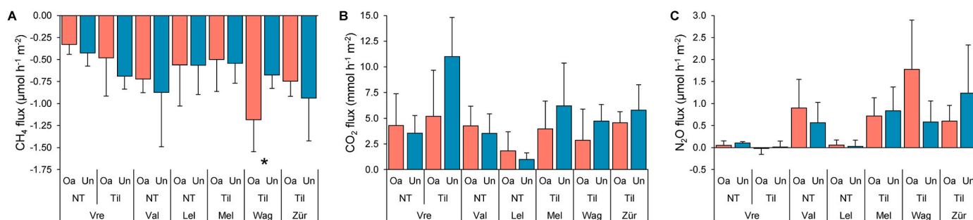
Fig. 2. Greenhouse gas fluxes (CH 4 (A), CO 2 (B), and N 2 O (C); mean \pm SD; n = 4-6 ) at visited field sites (Vre – Vredepeel; Val – Valthermond; Lel – Lelystad; Mel – Melle; Wag – Wageningen; Zür – Zürich) varying in agricultural practice (NT – no-tillage; Til – tillage) and treatment (Oa – organic-amended; Un – unamended). Significant differences are indicated with an asterisk (paired t -test; p \leq 0.05 ).
