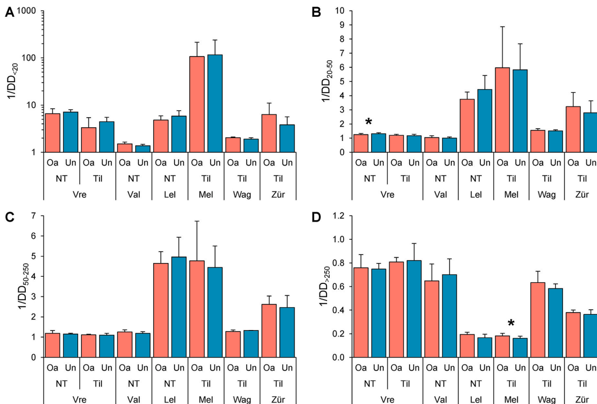
Fig. 3. The 1/DD ratio (mean \pm SD; n = 4-6 ), indicating the presence of non-water-stable aggregates, for size classes <20 \mu\text{m} (A), 20-50 \mu\text{m} (B), 50-250 \mu\text{m} (C), and >250 \mu\text{m} (D) of soils of visited field sites (Vre – Vredepeel; Val – Valthermond; Lel – Lelystad; Mel – Melle; Wag – Wageningen; Zür – Zürich) varying in agricultural practice (NT – no-tillage; Til – tillage) and treatment (Oa – organic-amended; Un – unamended). Significant differences are indicated with an asterisk (paired t -test; p \leq 0.05 ).
