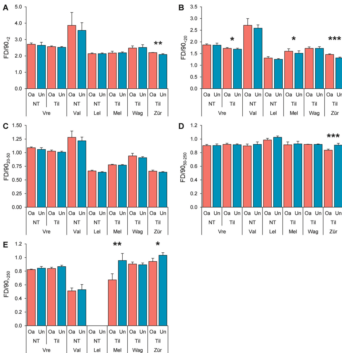
Fig. 5. The FD/90 ratio (mean \pm SD; n = 4\text{--}6 ), indicating the presence of persistent stable aggregates, for size classes <2\ \mu\text{m} (A), <20\ \mu\text{m} (B), 20\text{--}50\ \mu\text{m} (C), 50\text{--}250\ \mu\text{m} (D), and >250\ \mu\text{m} (E) of soils of visited field sites (Vre – Vredepeel; Val – Valthermond; Lel – Lelystad; Mel – Melle; Wag – Wageningen; Zür – Zürich) varying in agricultural practice (NT – no-tillage; Til – tillage) and treatment (Oa – organic-amended; Un – unamended). Significant differences are indicated with an asterisk (paired t -test; * p < 0.05 , ** p < 0.01 , *** p < 0.001 ).
