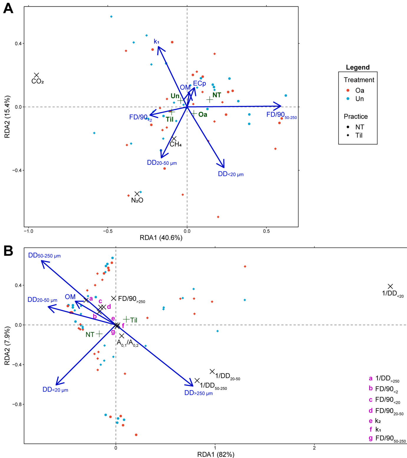
Fig. 6. RDA on variables explaining the variability observed in the soil GHG fluxes (A) and the soil aggregate stability (B), obtained using the soil parameters dry dispersion for all size classes ( DD_{<20 \mu m} ; DD_{20-50 \mu m} ; DD_{50-250 \mu m} ; DD_{>250 \mu m} ), organic matter content (OM), and pore water conductivity (ECp); the aggregate stability parameters 1/DD for all size classes ( 1/DD_{<20} ; 1/DD_{20-50} ; 1/DD_{50-250} ; 1/DD_{>250} ), k_1 , k_2 , A_{0,1}/A_{0,2} , and the FD/90 for all size classes ( FD/90_{<2} ; FD/90_{<20} ; FD/90_{20-50} ; FD/90_{50-250} ; FD/90_{>250} ); and the management variables treatment (Un for unamended, Oa for organic-amended) and practice (NT for no-tillage, Til for tillage).
