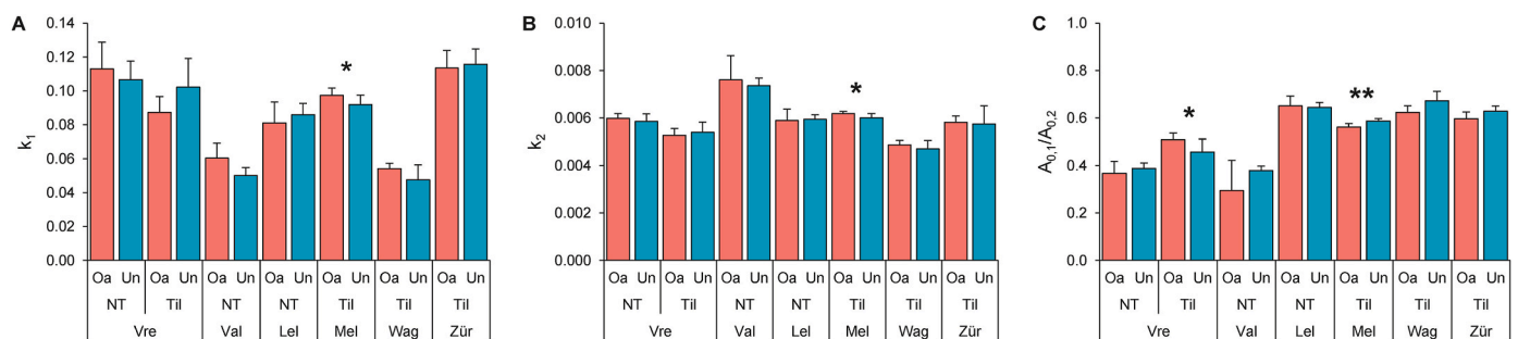
Fig. 4. The disintegration coefficient of weak aggregates k_1 (A), the disintegration coefficient of stable aggregates k_2 (B), and the ratio of weak versus stable aggregates A_{0,1}/A_{0,2} (C) (mean \pm SD; n = 4-6 ) of soils of visited field sites (Vre – Vredepeel; Val – Valthermond; Lel – Lelystad; Mel – Melle; Wag – Wageningen; Zür – Zürich) varying in agricultural practice (NT – no-tillage; Til – tillage) and treatment (Oa – organic-amended; Un – unamended). Significant differences are indicated with an asterisk (paired t -test; * p \leq 0.05 , ** p \leq 0.01 ).
